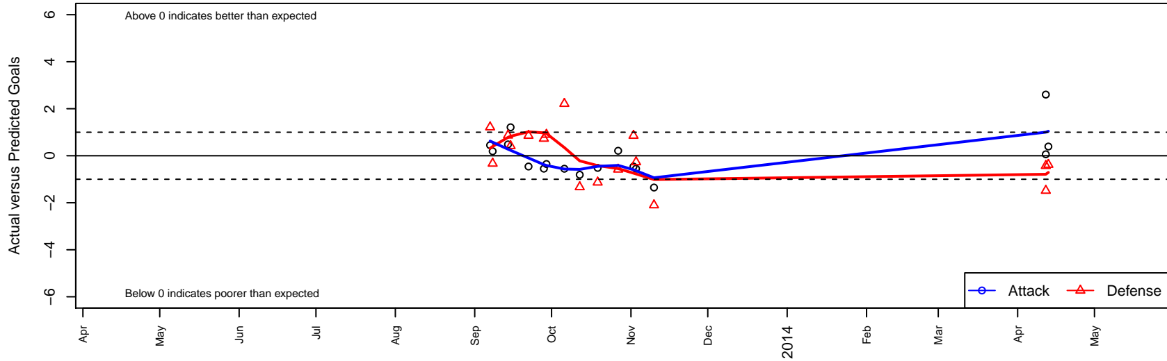
PCSC White B96 Dots are actual minus expected GF (blue circles) and GA (red triangles). Blue line is smoothed change in attack strength. Red is smoothed change in defense strength.
